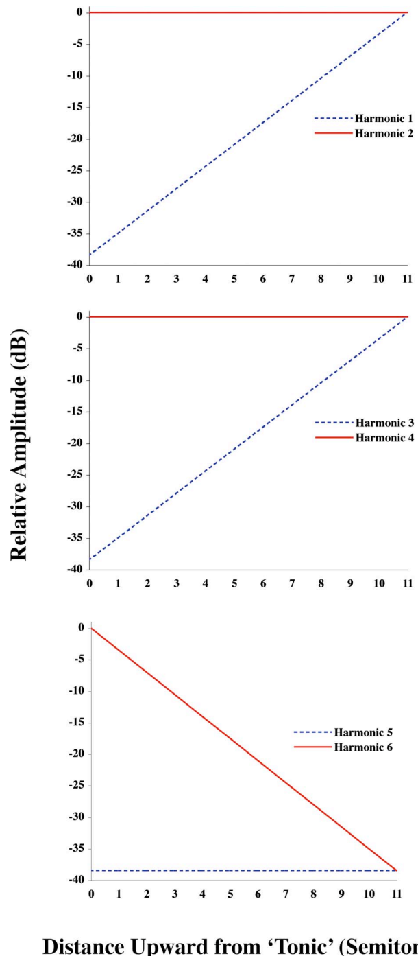
FIG. 3. (Color online) Progression of the relative amplitudes of harmonics 1 and 2, harmonics 3 and 4, and harmonics 5 and 6 as F_0 moves upward from the “tonic.”
